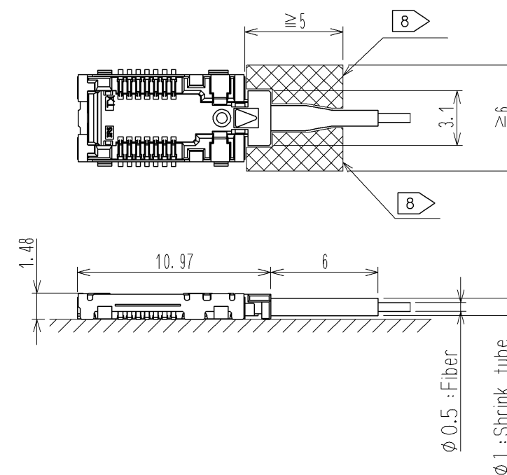
Dimensions of engaged connector (Scale : FREE)
