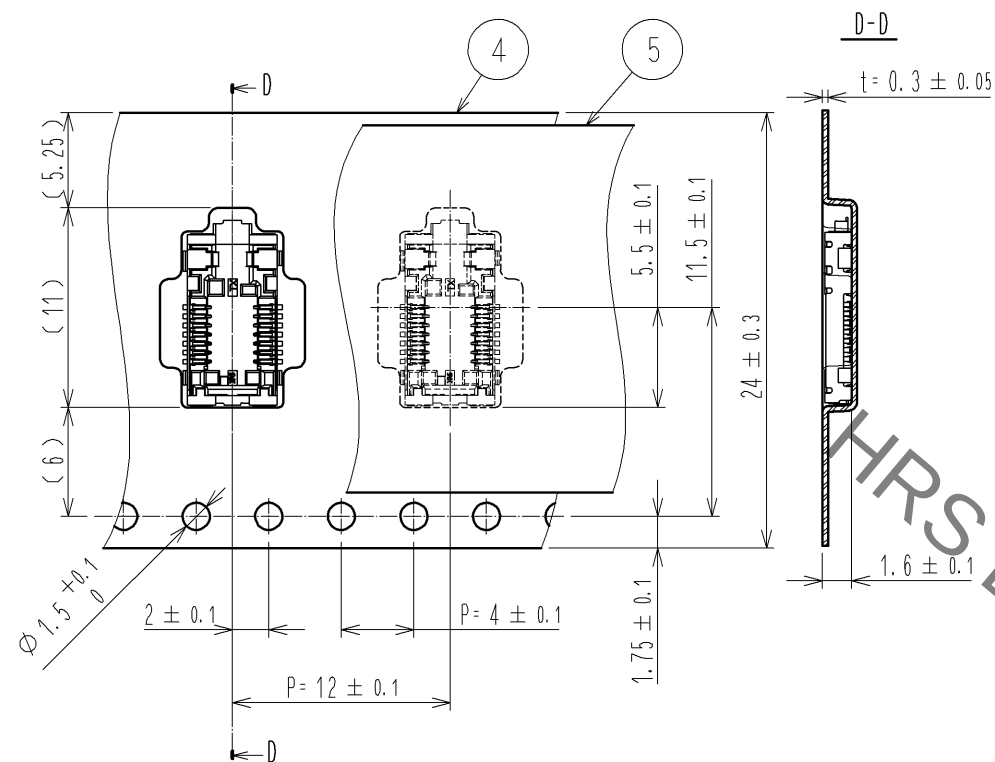
Taping direction (Scale : FREE)
