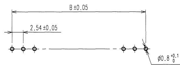
RECOMMENDED PC BOARD HOLE PATTERN
