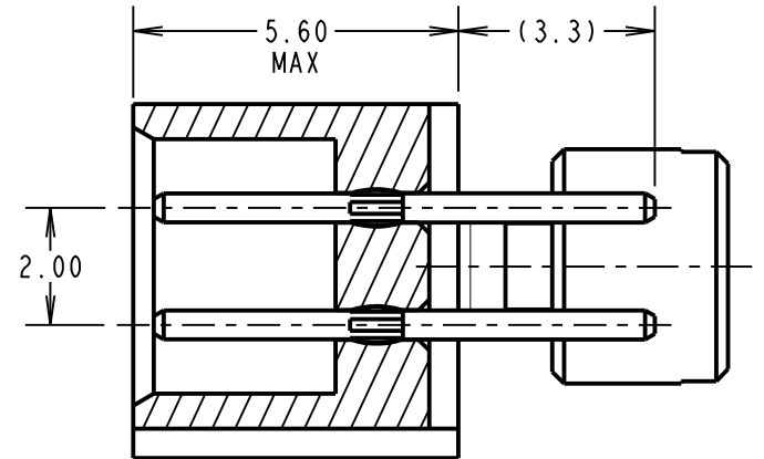
SECTION X-X
