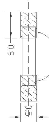
Figure 1. IN-S85CS5Y Solder Pattern
