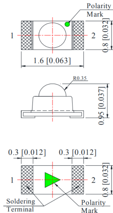
Figure 2. IN-S63WT Package Dimensions
