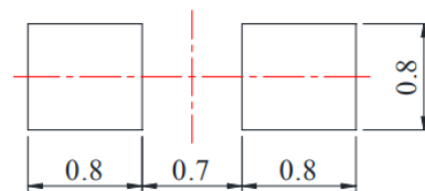
Figure 1. IN-S63WT Solder Pattern
