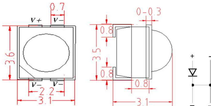
Figure 2. IN-P36BTFY Package Dimensions
