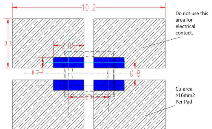
Figure 1. IN-P36BTFY Solder Pattern
