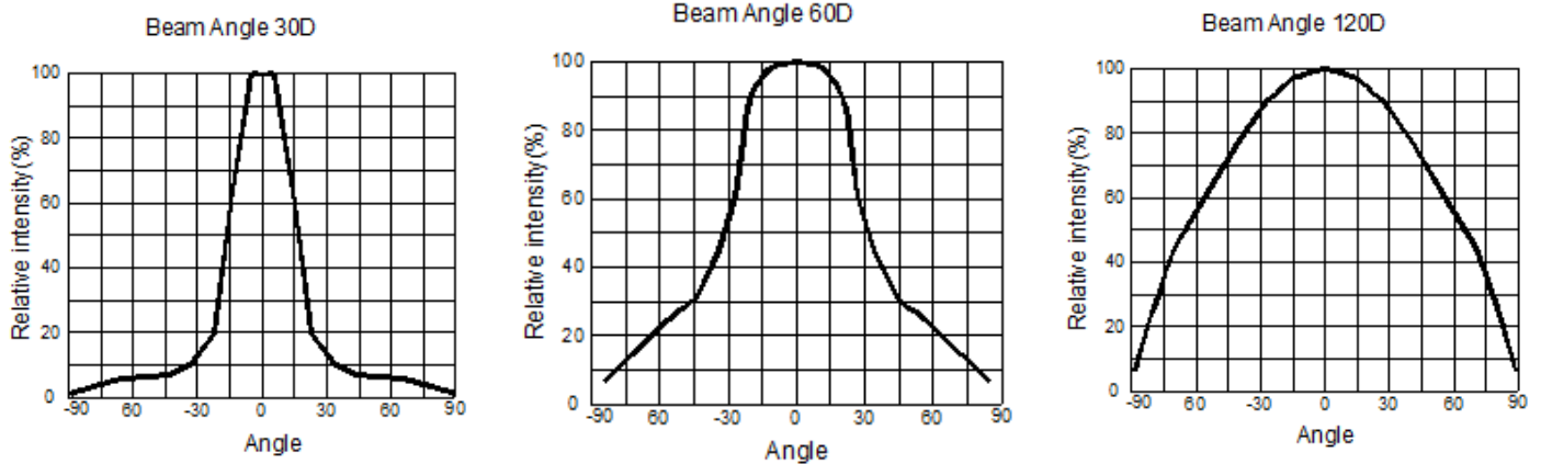
Beam Angle (2 \theta 1/2)
