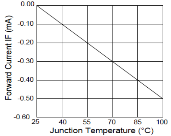
Forward Voltage Shift VS. Tj
