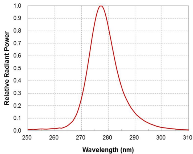
Relative Spectral Power Distribution
