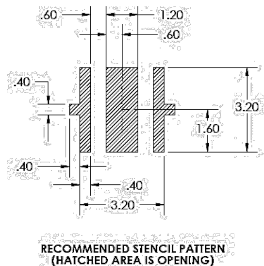
Figure 1. INV-Q39CTSIR Recommended Solder Pattern
