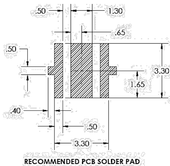
Figure 1. INV-Q39CTSIR Recommended Solder Pattern
