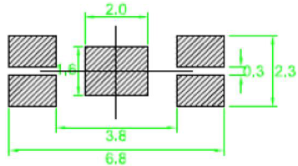
Figure1. INV-P53CTRIR Solder Pattern
