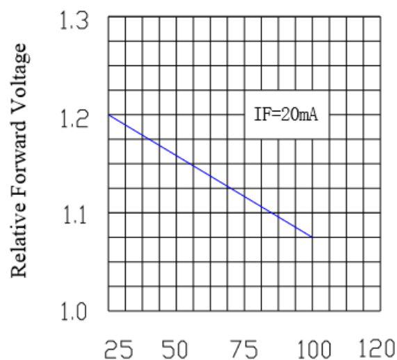
Forward Voltage & Ambient Temperature( ^{\circ} C)
