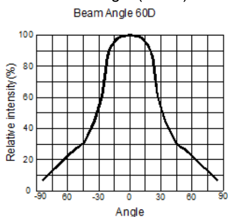
Beam Angle (2θ1/2)
