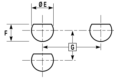
Jam nut receptacle back panel mounting
