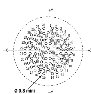
79 contacts size 22D
