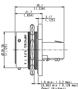
RJF6 7 x 1 X Straight Female RJ45 Sortie RJ45 droite
