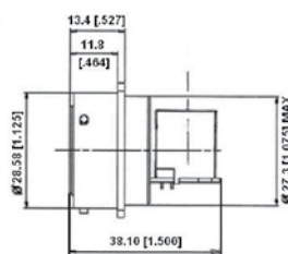
RJF 21 RA x Right Angle Female RJ45 Sortie RJ45 coudée
