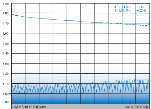
Typical VSWR
