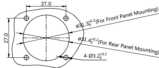
PANEL CUT OUT REFERENCE
