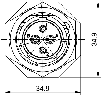
MASTER KEYWAY
