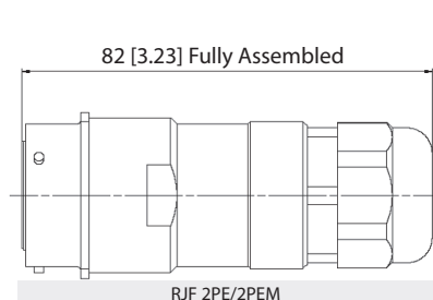
RJF 2PE/2PEM
