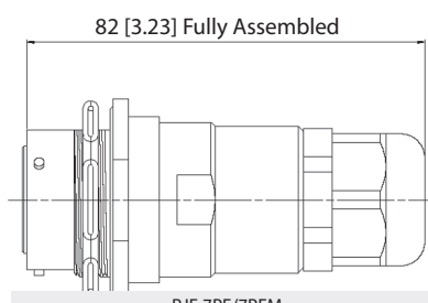
RJF 7PE/7PEM
