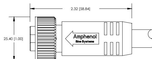
FIG 2: Female, Plug, Mini, Straight, Internal Threads
