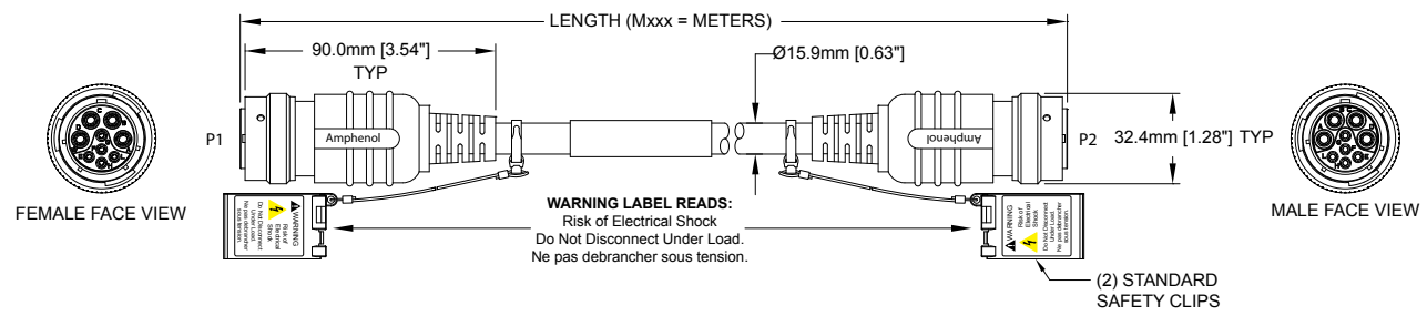
FIG 3: Male Plug to Female Plug, Straight, 9 Position
