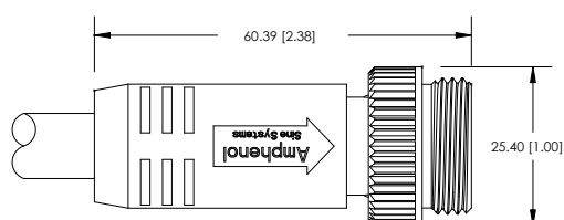
FIG 1: Male, Mini, Plug, Straight, External Threads
