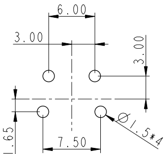
4Pin Male Connector Male Pin PCB Layout
