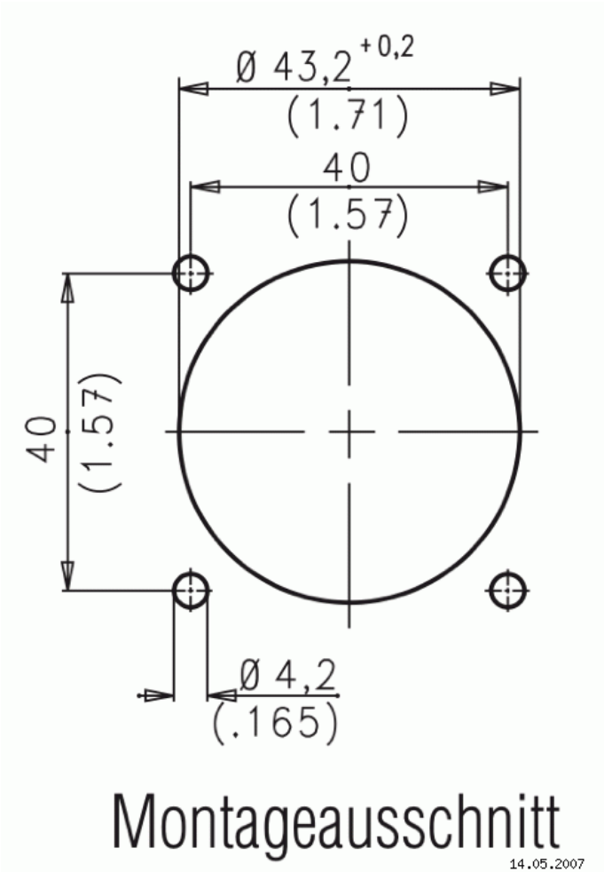
Panel cutout
