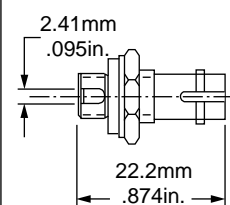
Part number: 88-FJ-7B, coupling nut on ST side
