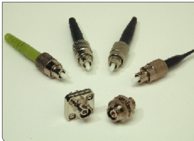
FC Connector & Adapter Family
