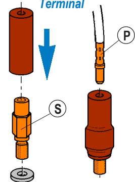
Borne Terminal
