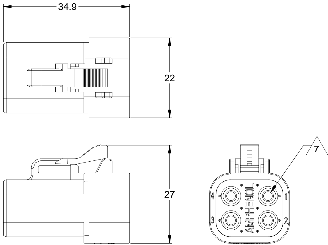
REFERENCE DIMENSIONS - ASSEMBLED PLUG
