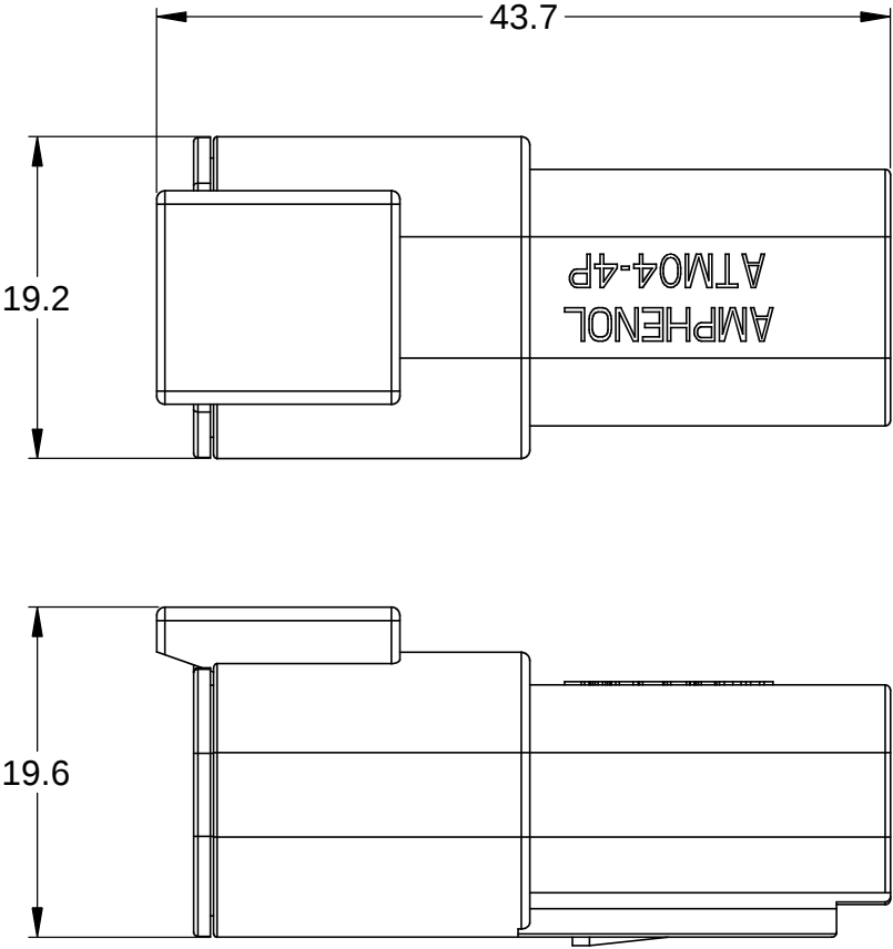
REFERENCE DIMENSIONS - ASSEMBLED
