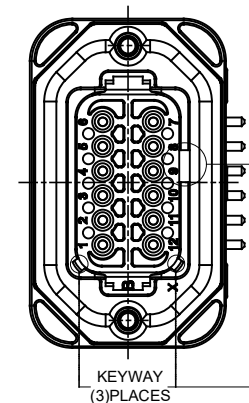
P/N AT13-12PB-BM1X KEY-B CONFIGURATION STANDARD COLOR: BLACK
