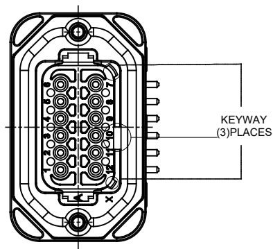
P/N AT13-12PA-BM1X KEY-A CONFIGURATION STANDARD COLOR: GREY
