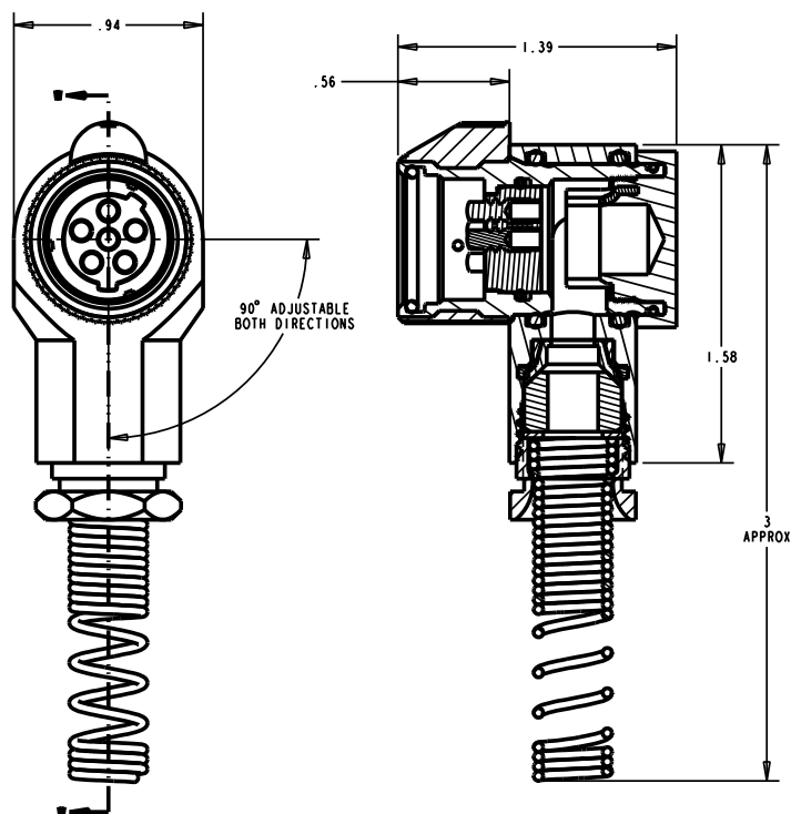
SECTION W-W
