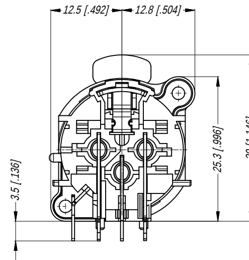
MIN MOUNTING PITCH (1:1)
