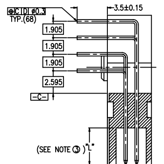
SECTION "E-E" (5/1)
