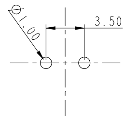
Recommend PCB Layout
