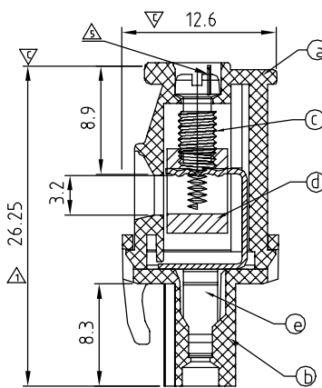
SECTION P-P
