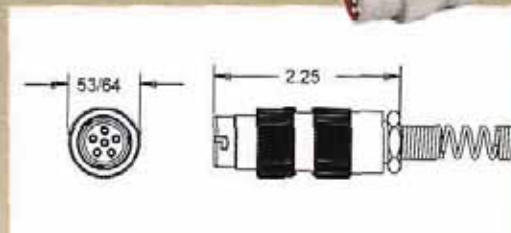
AJ-156 (M55116/12)
