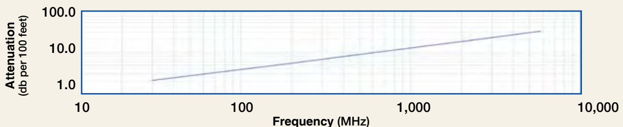
Attenuation vs. Frequency (typical)
