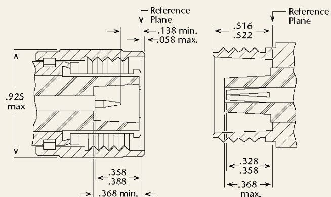
Plug (male)
