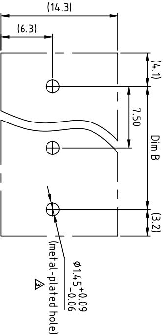
P.C.B LAYOUT Top view
