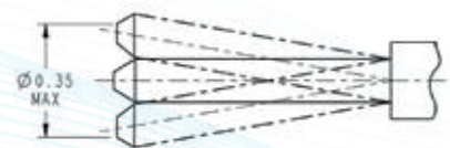
DETAIL A
