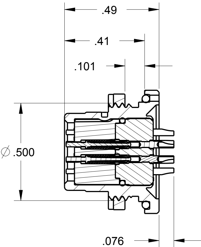
SECTION Z-Z
