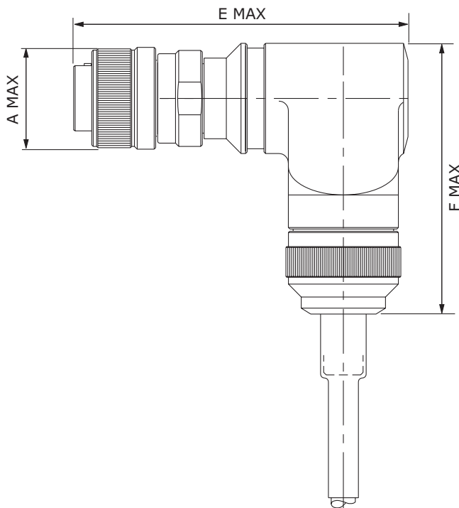
M28876/9 Plug with 90° Backshell
