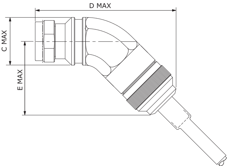
M28876/28 45° Backshell
