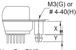
H or G + RM5 Standoff + Boardlock
