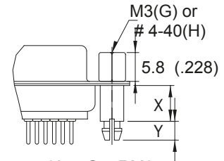
H or G + RM8 Front Screwlock with Standoff + Boardlock
