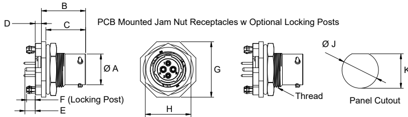
PCB Mounted Jam Nut Receptacles w Locking Posts - Dimensions (in mm)
