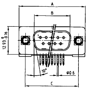
Plug connector
