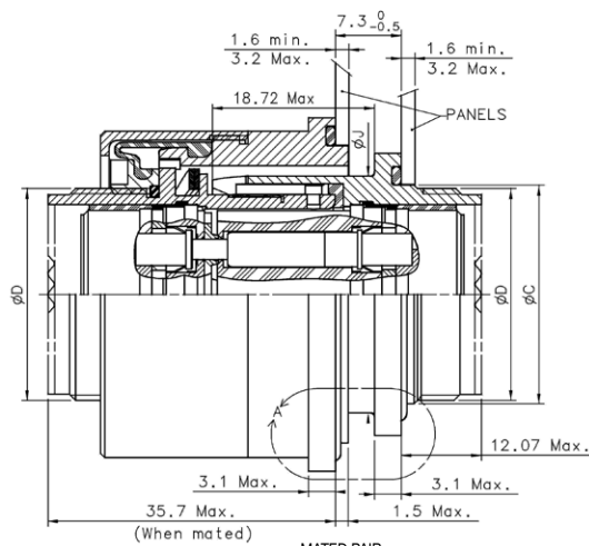
MATED PAIR
