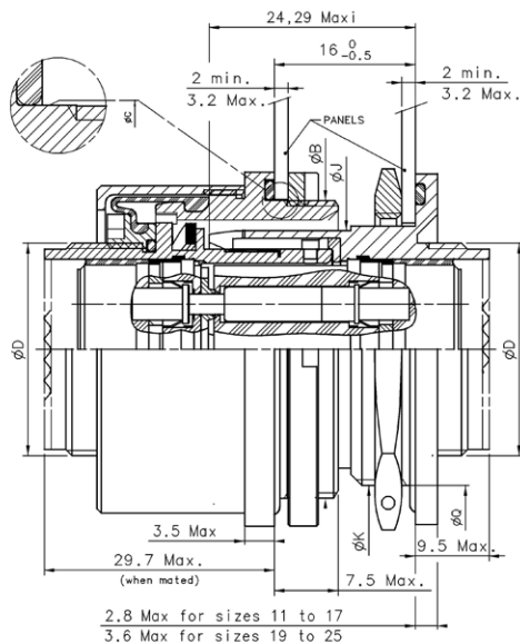
MATED PAIR
