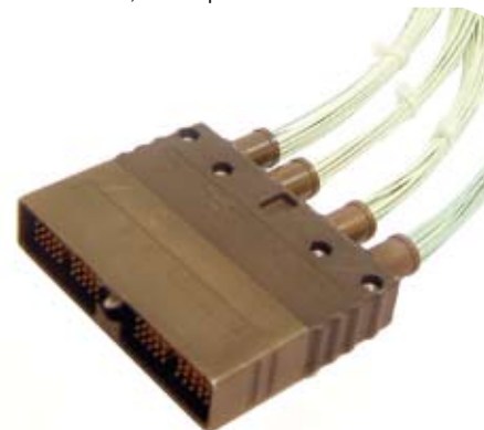
4 modules metallic plug, with cadmium plating, fitted with wired modules, a backshell and 4 chimneys.
