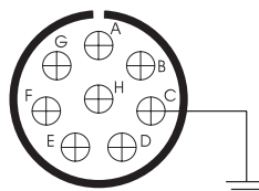
8 Contact Shell Size 18
