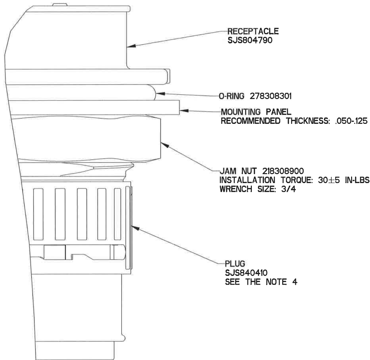
MOUNTING INSTRUCTIONS
