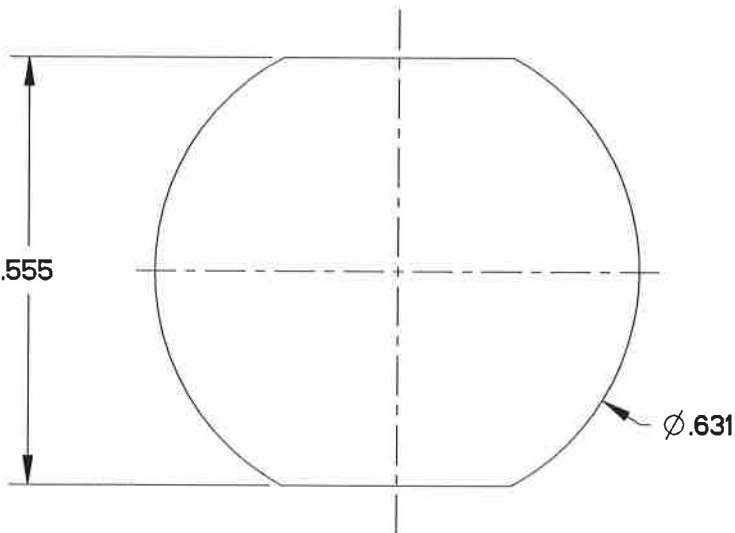
MOUNTING PANEL CUT OUT
