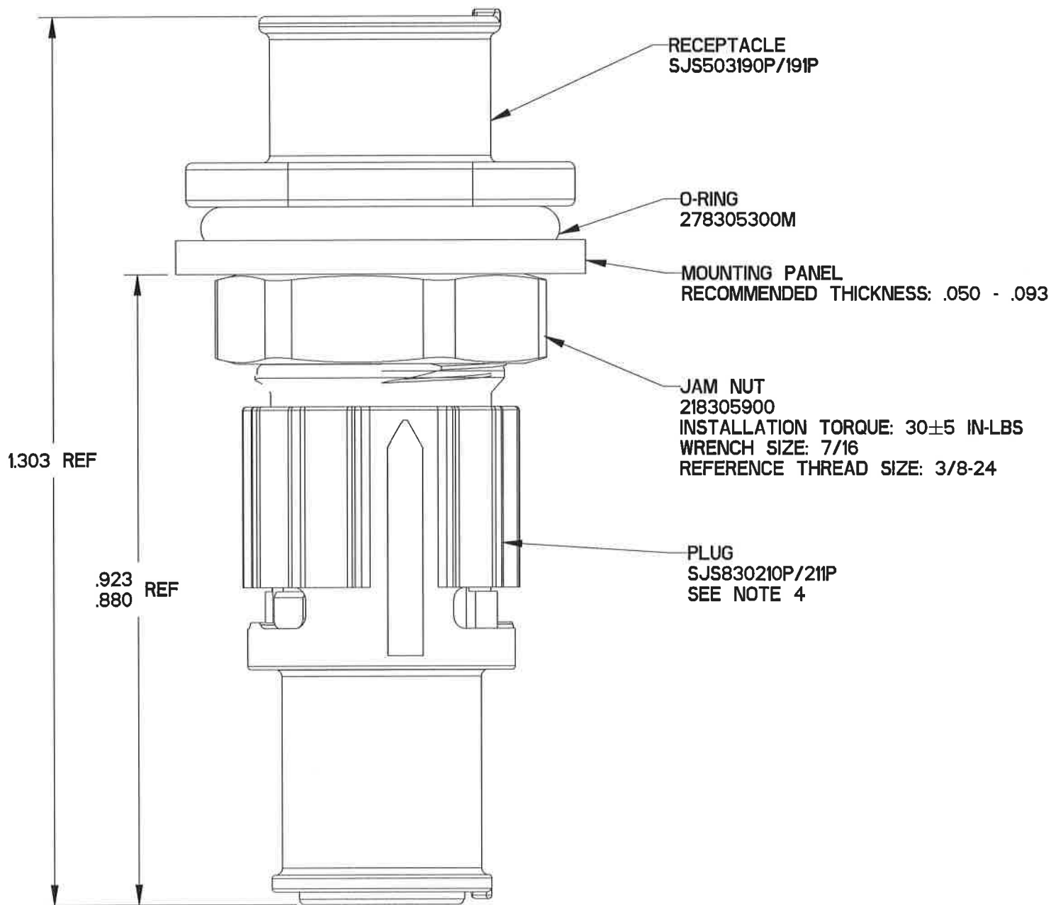
MOUNTING INSTRUCTIONS
