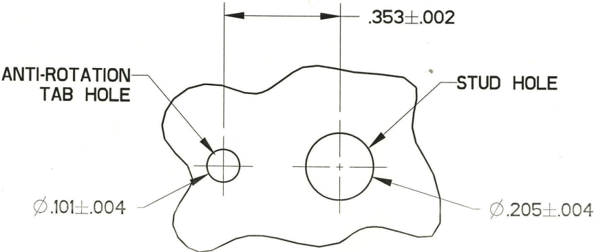
MOUNTING HOLE CONFIGURATION
