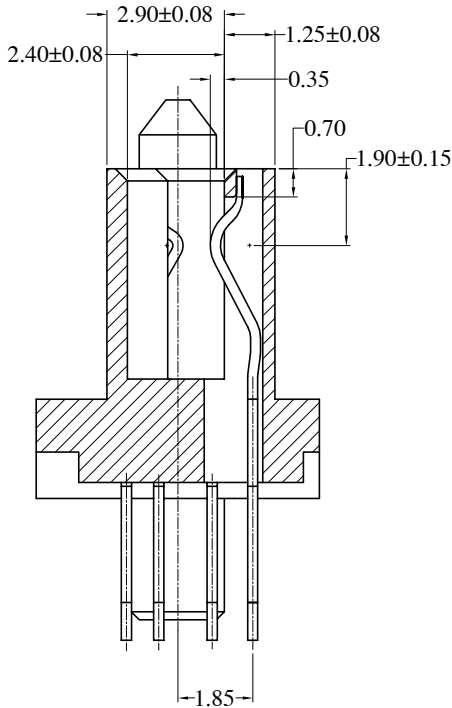
SECTION B-B
