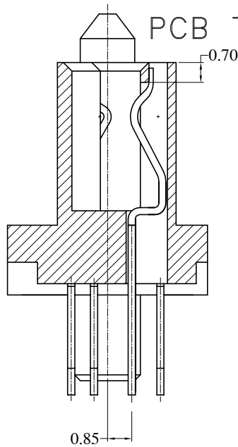
SECTION E-E
