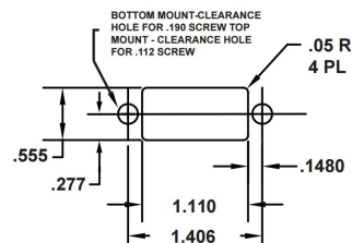
Recommended Mounting Panel Cutout
