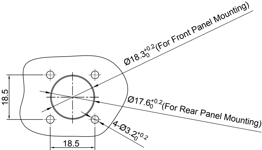
PANEL CUT OUT REFERENCE
