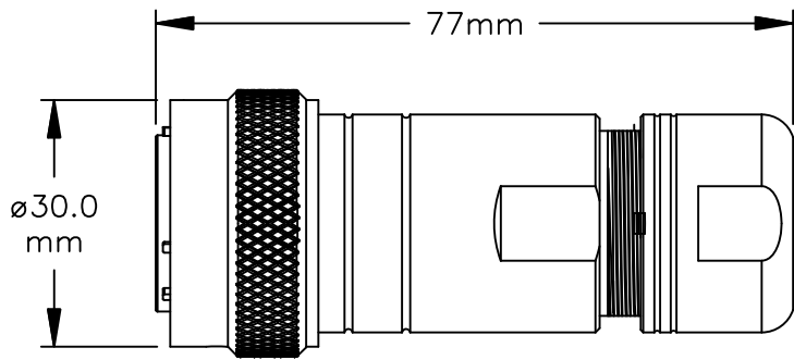
ASSEMBLED VIEW
