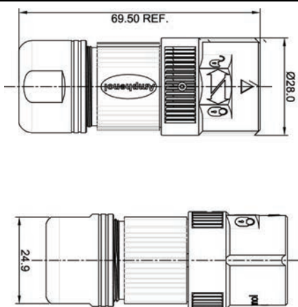
Plug
